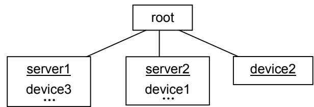
Figure 2: Decomposition tree after the adaptation.
