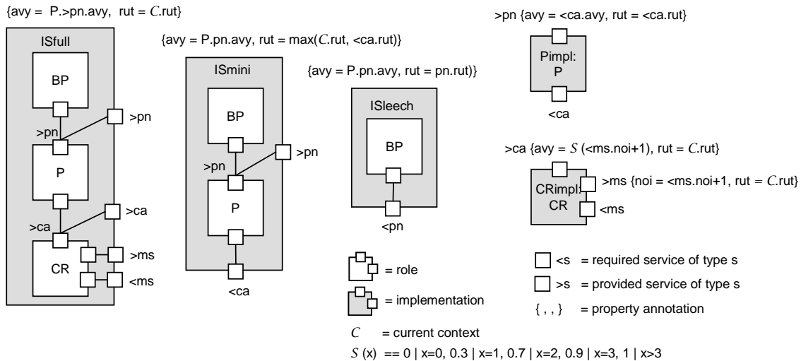
Figure 1. InstantSocial partial architecture model
