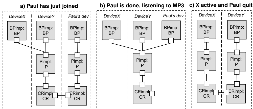
Figure 2 Configurations of InstantSocial
